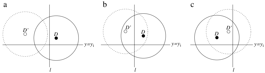
Fig. 1. Three scenarios for a red disk D to dominate another red disk D' at a vertical line l .
