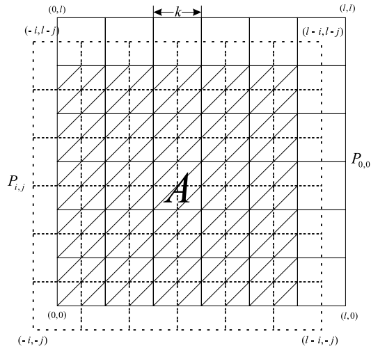
Fig. 1. Two partitions P_{0,0} and P_{i,j} with the shadow area A . The solid lines represent partition P_{0,0} and the dashed lines represent partition P_{i,j} .
