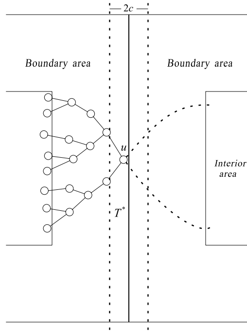
Fig. 3. The tree T^* and the vertex u .
